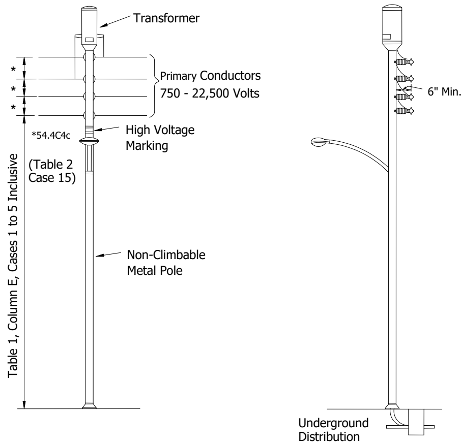
Figure 54-2 Partial Underground
