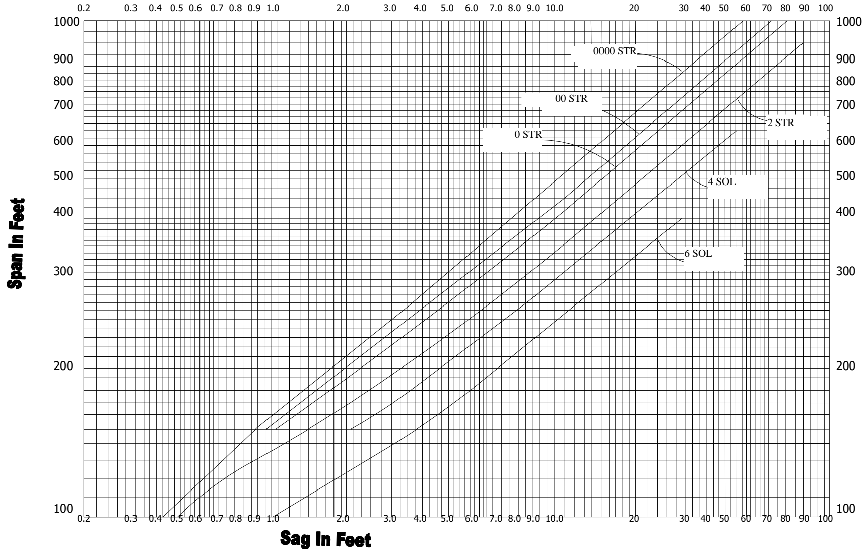
Chart No. 4 Heavy Loading Sags at 60°F and No Wind Bare Copper - Medium Hard Drawn
